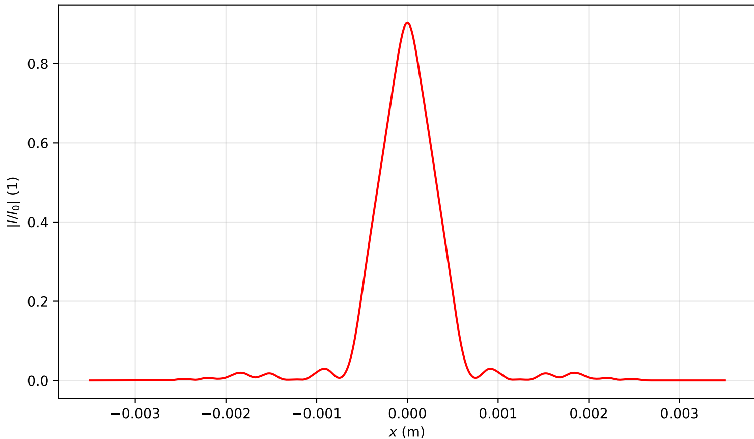
Intensity profile I(x, y = 0, z = 2.627)/I_0 , \text{Pin}=2.5\text{Pcr} , artificial time
